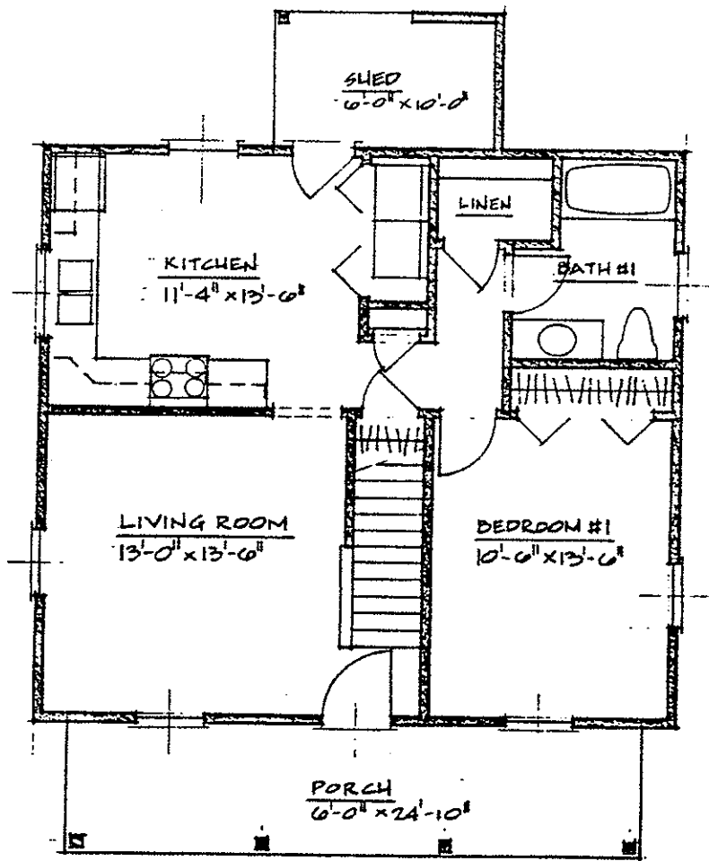
FIRST FLOOR PLAN 1/8" = 1'-0"
